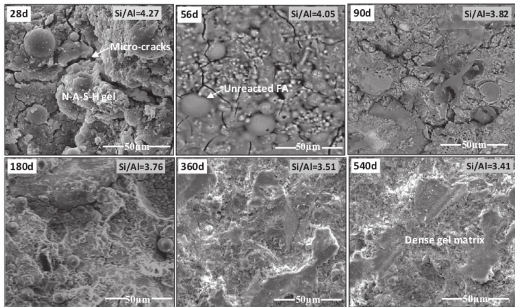
Fig. 7. Microstructural development of FAGP concrete.
