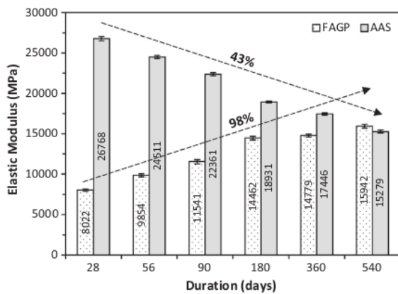
Fig. 3. Elastic modulus development vs time.
