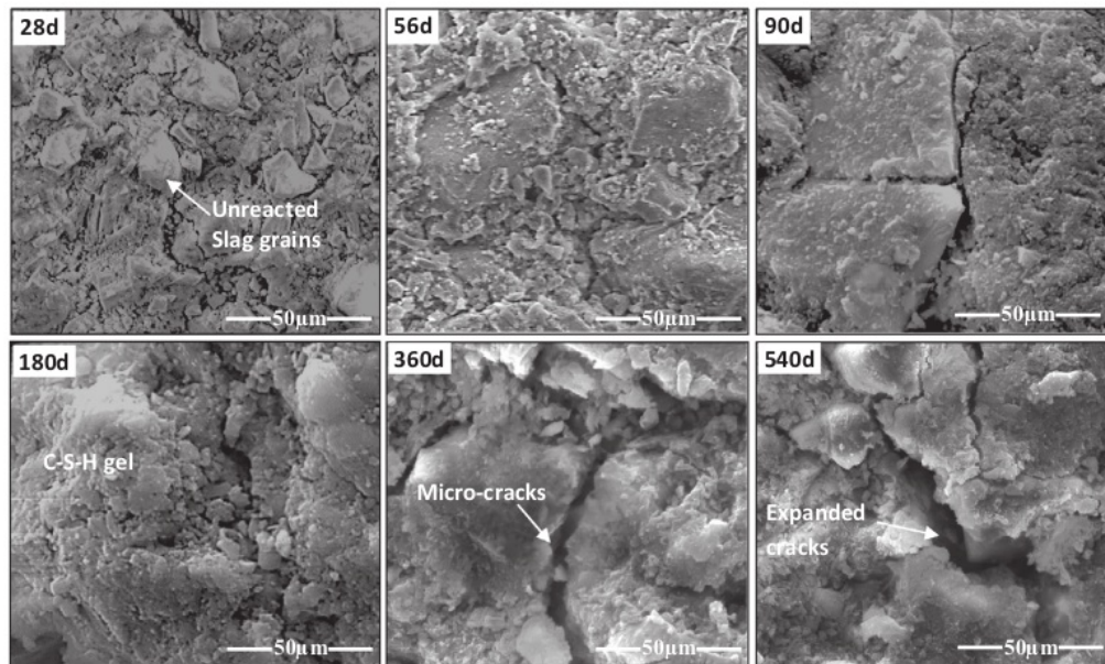
Fig. 8. Microstructural development of AAS concrete.
