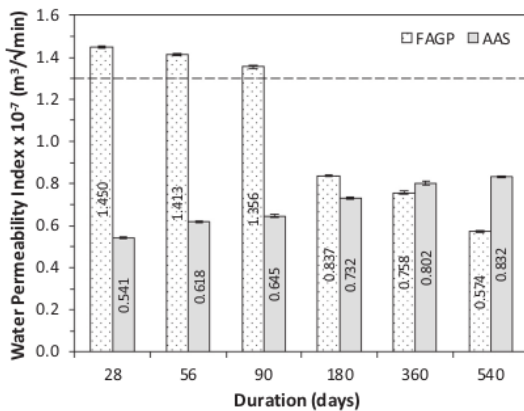
Fig. 5. Water permeability index vs. time.
