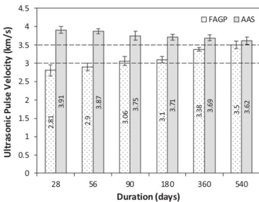
Fig. 6. Ultrasonic pulse velocity vs. time.
